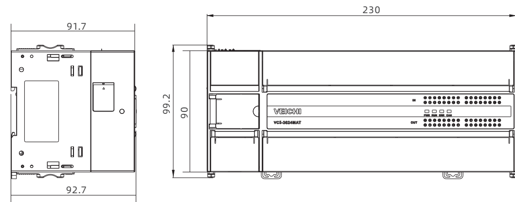
VC3/VC5 long point master module size diagram
