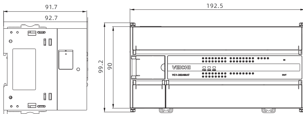
VC1 main module long point size diagram
