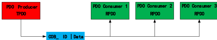
Figure 11- 5 PDO transmission mode
