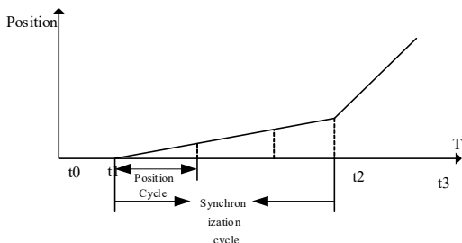
Figure 11- 29 Interpolation position diagram
