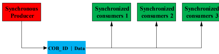
Figure 11- 8 Synchronization transmission mode
