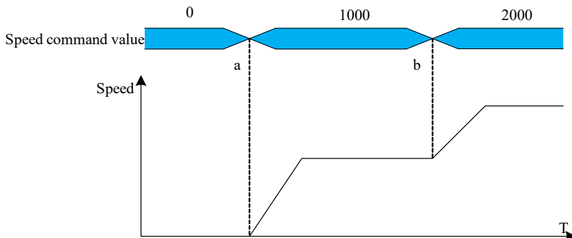
Figure 11- 21 Profile speed mode running time sequence diagram
