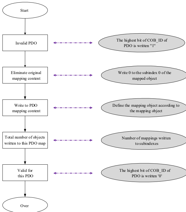
Figure 11- 4 PDO mapping configuration process
