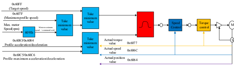
Figure 11- 17 Profile velocity mode control diagram
