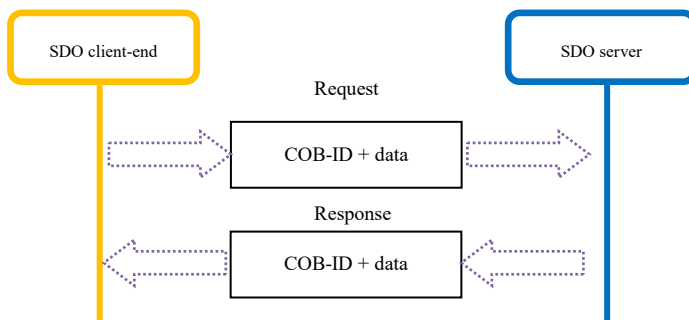
Figure 11- 3 SDO client-end read and write the object dictionary in SDO server
