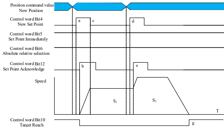
Figure 11- 15 Timing sequence of relative position command value in immediate change mode
