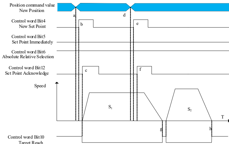
Figure 11- 16 Timing sequence for non-immediate change mode of relative position command value
