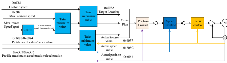
Figure 11- 11 Profile position mode control diagram
