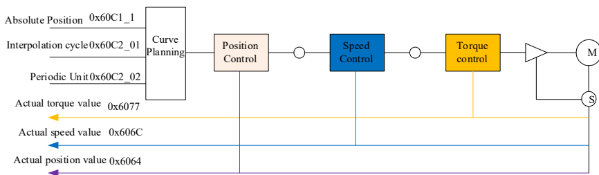
Figure 11- 27 Interpolation mode control block diagram
