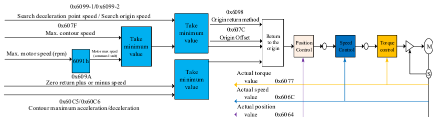
Figure 11- 23 Homing method control diagram
