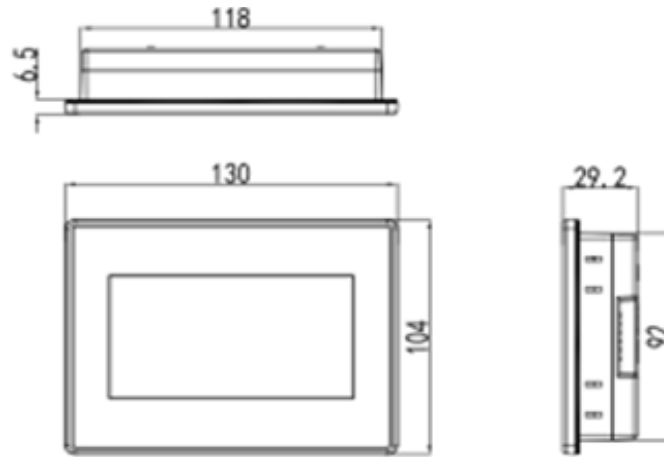
Overall Dimensions
