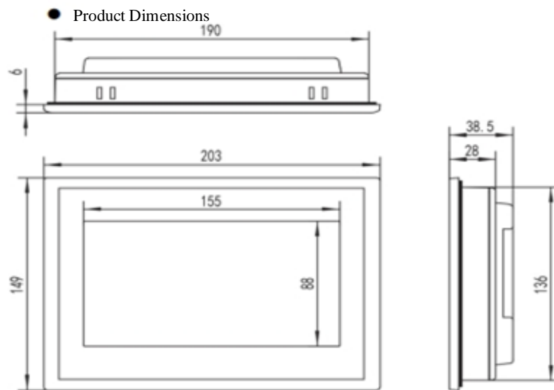
Overall Dimensions
