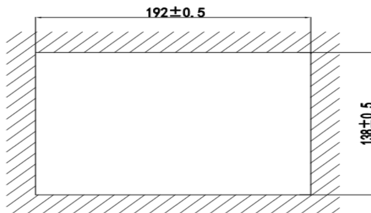
Embedded installation hole size: 192*138(mm)
